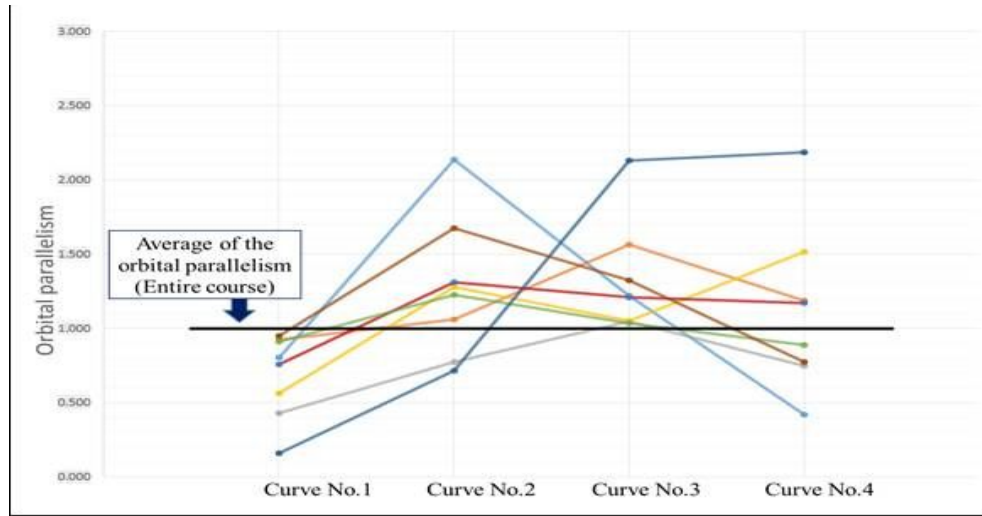
Figure 7: Orbit Parallelism of Each Curve Section Divided by Orbit Parallelism of the Entire Course
