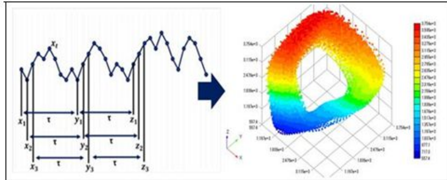
Figure 3: Embedding Theorem and Attractor
